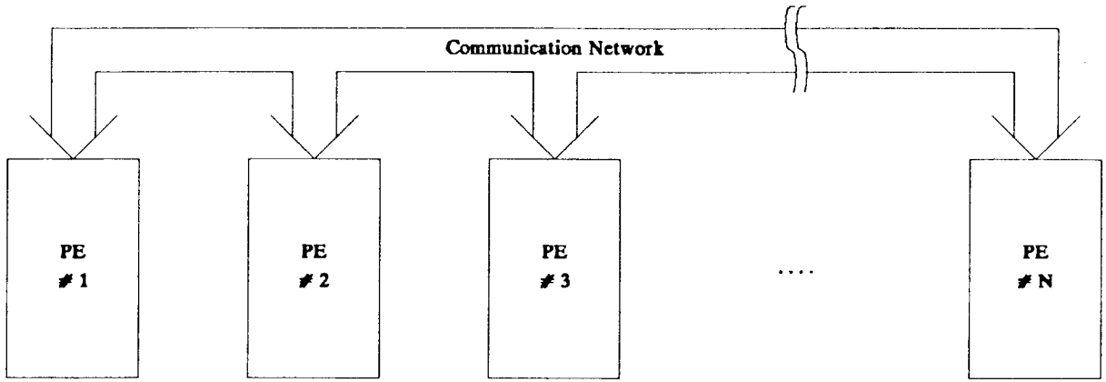
Figure 8. Organization of the parallel reduction machine.
