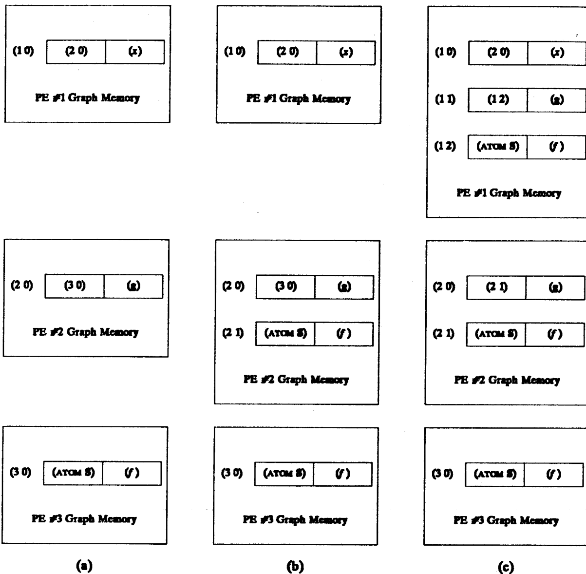
Figure 6. First Steps in Reducing S f g x
